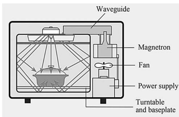
Fig.7.1. Schematic diagram of a typical microwave.
